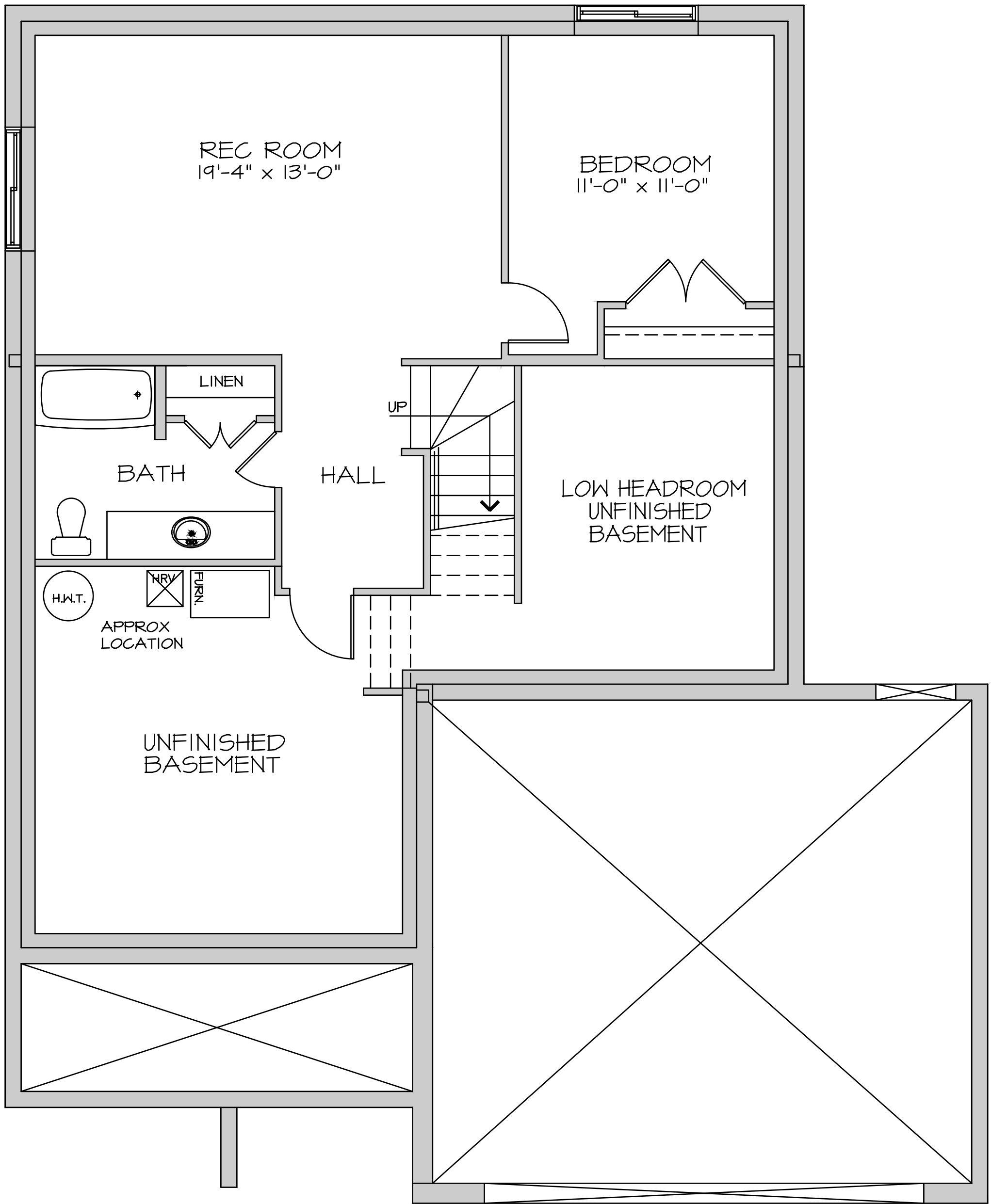
BASEMENT PLAN FINISHED AREA 560 SQ. FT.
